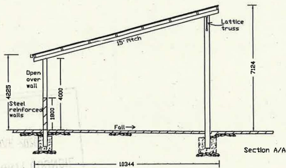
Plan/Section A/A
