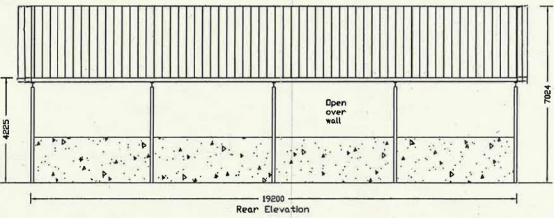
Rear Elevation
