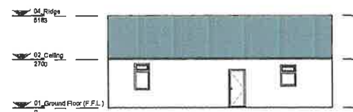
Rear Elevation - 1:100
