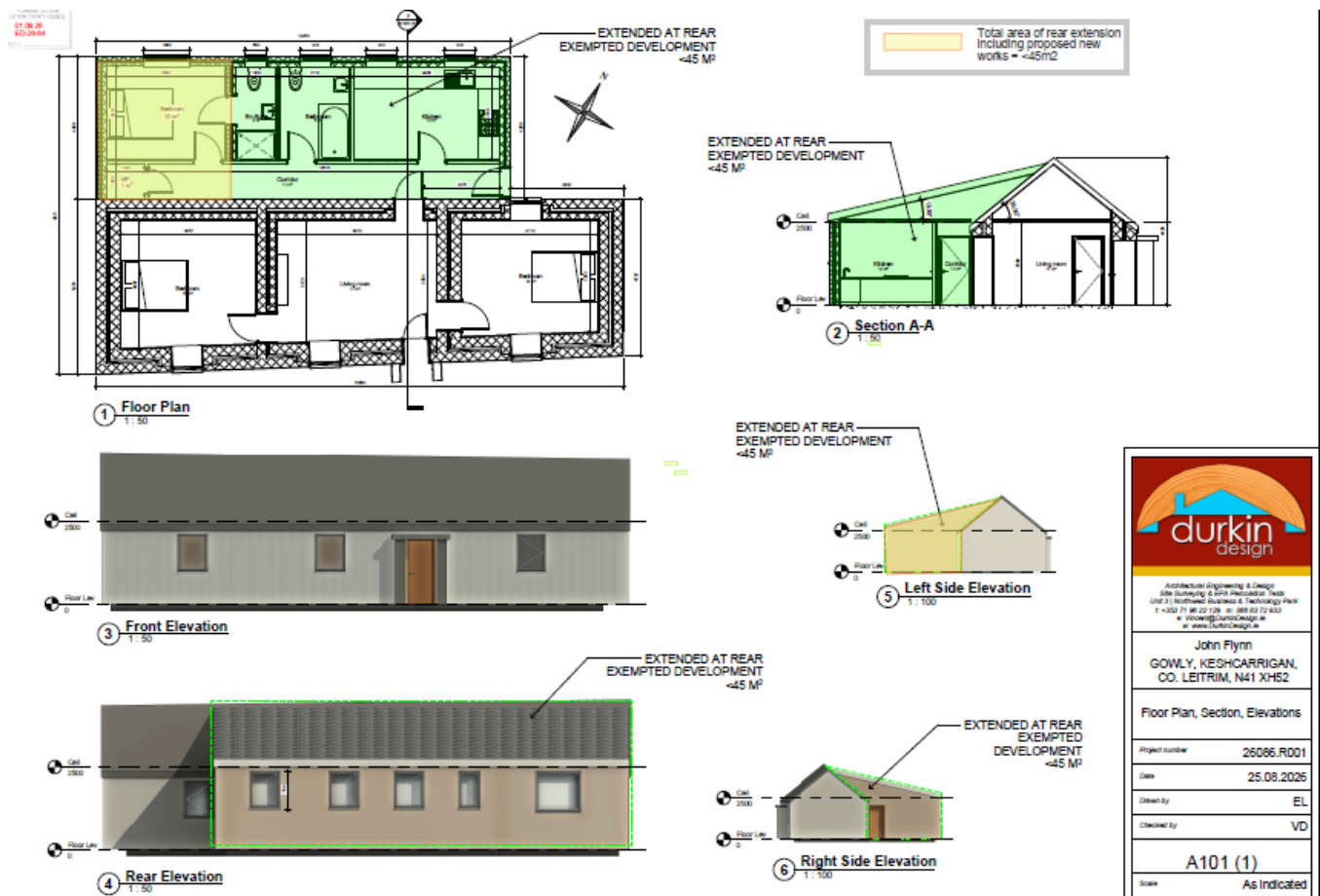
Fig. 11: Submitted drawing of proposed extension
