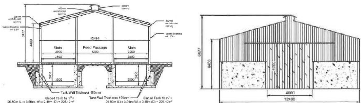
Fig. 2 Proposed Slatted Shed Dimensions
