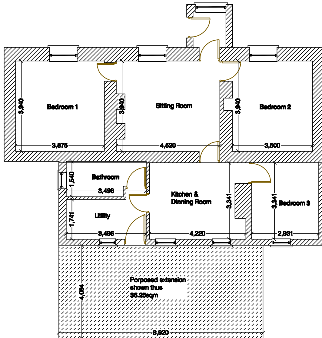
Existing Floor Plan with dimensions overlaid with proposed extension Plan scale 1:100 on A4
