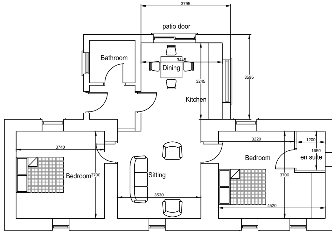
PLAN scale 1:100 on A4
