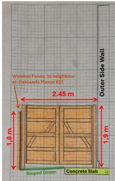
Fig. 8: Proposed dual wooden gates to be installed
