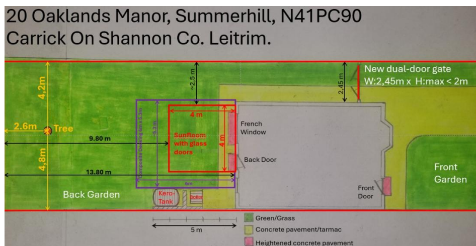
Fig. 6: Proposed layout plan for conservatory/ sunroom
