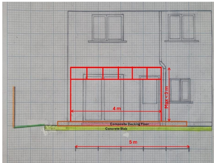
Fig. 5: Proposed conservatory/ sunroom
