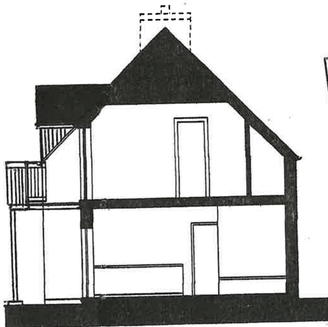
SECTION CC
