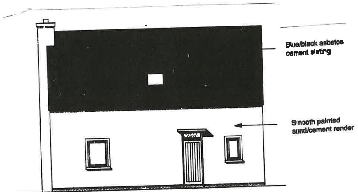
REAR ELEVATION
