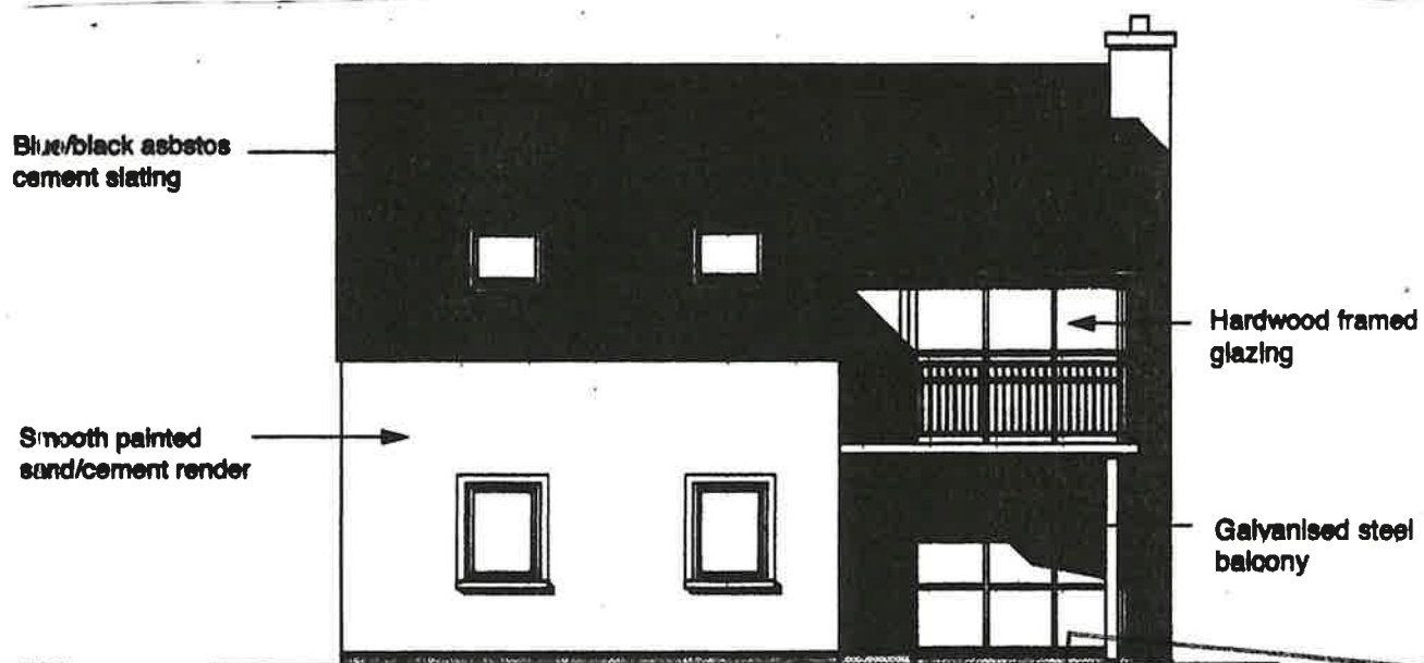
FRONT ELEVATION
