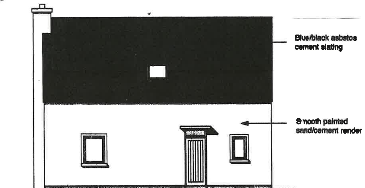
REAR ELEVATION
