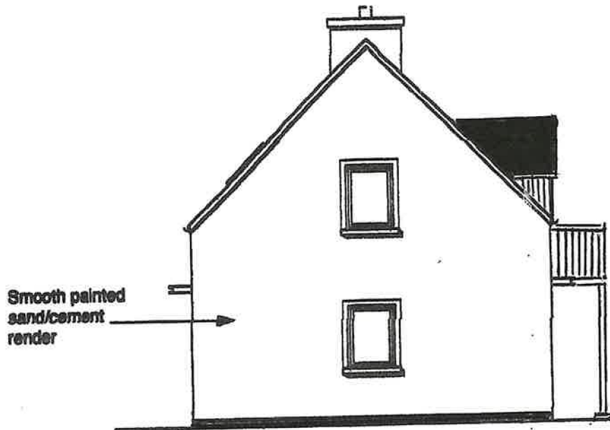
SIDE ELEVATION
