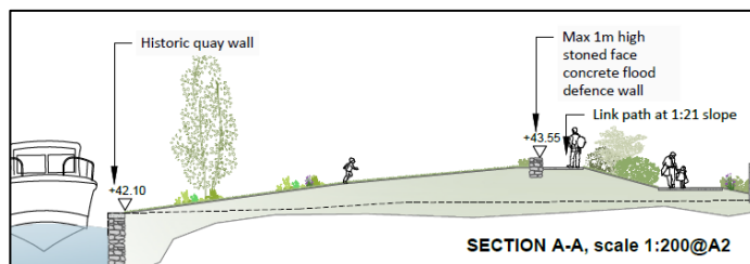
Draft proposed cross section at Bridge Park.
