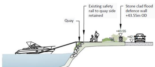
Draft proposed cross section at Leitrim Quay.
